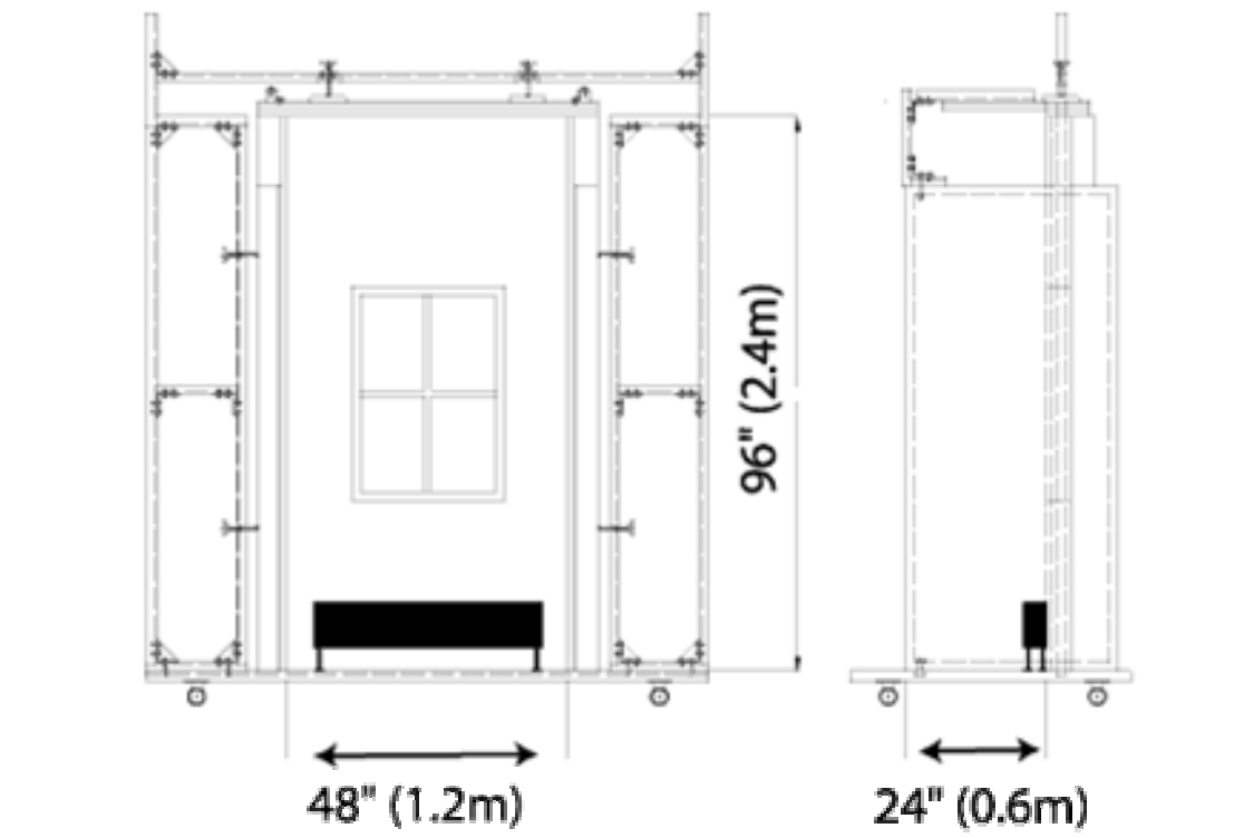
Figure 1. Schematic of the Wall Assembly Test Module used for evaluating the fire performance of a window.
